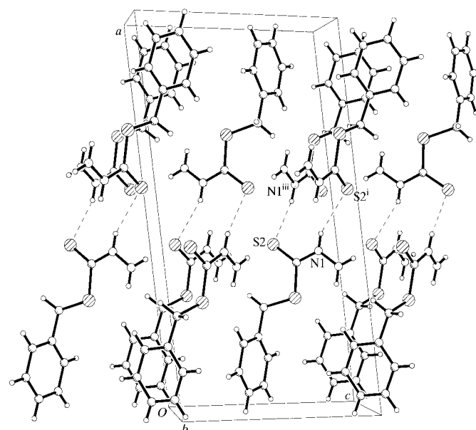
Figure 2 The packing of the molecules of (I) viewed down the b axis [symmetry codes: (i) 1 - x, y + \frac{1}{2}, \frac{3}{2} - z ; (iii) 1 - x, y - \frac{1}{2}, \frac{3}{2} - z ].
